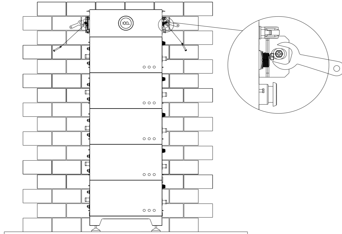
Figure 4.10 Assembling the bracket
