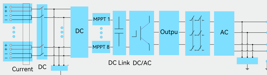
Topology Diagram
